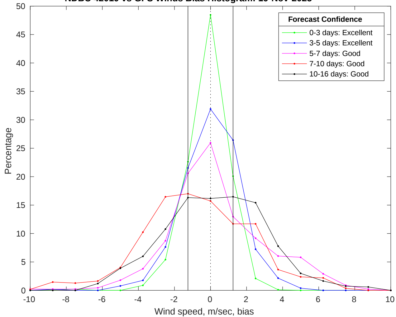
NDBC 42019 vs GFS Winds Bias Histogram: 19-Nov-2025
