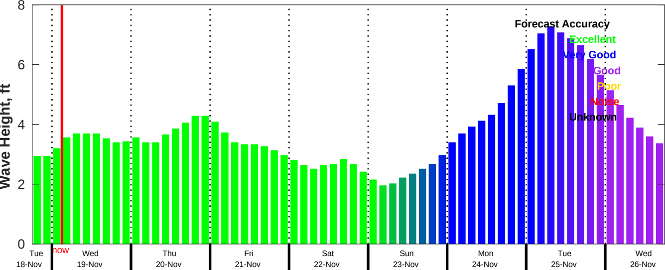
CMEMS Wave Forecast for NDBC 42019 from 18-Nov-2025 18:00:00 to 26-Nov-2025 18:00:00
