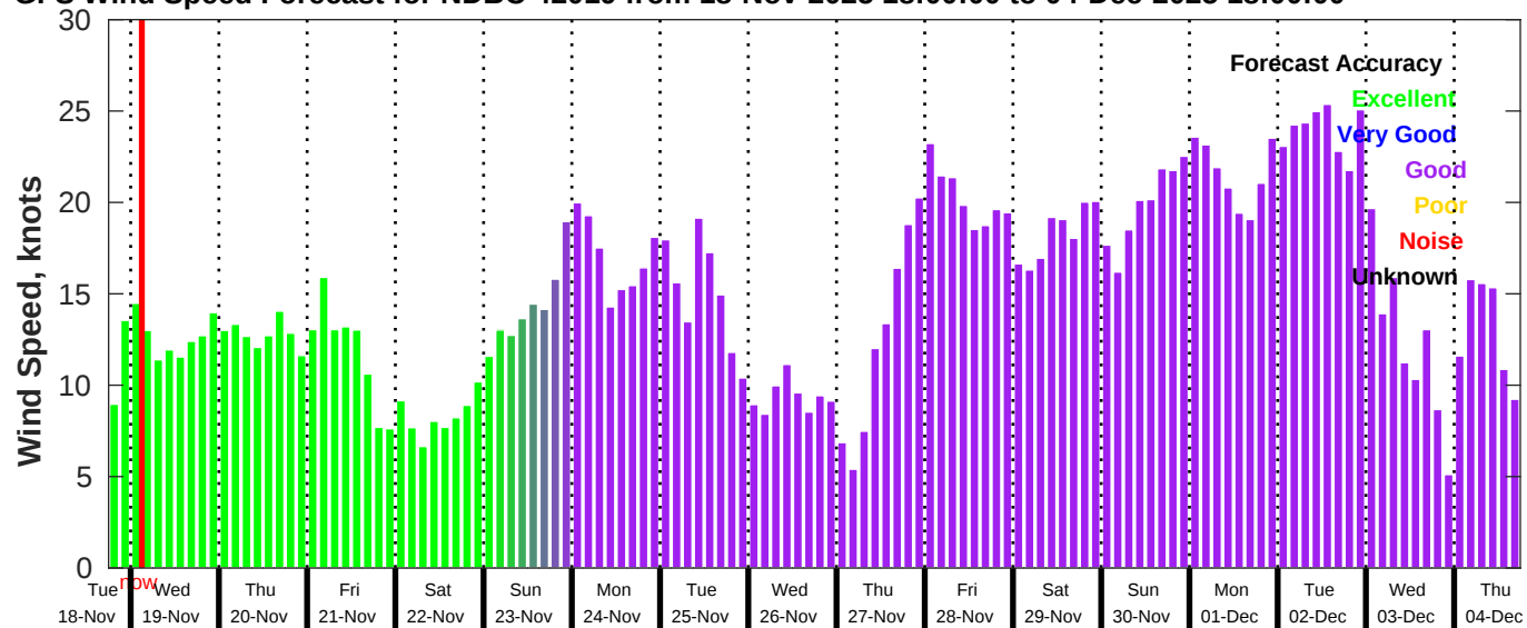
GFS Wind Speed Forecast for NDBC 42019 from 18-Nov-2025 18:00:00 to 04-Dec-2025 18:00:00
