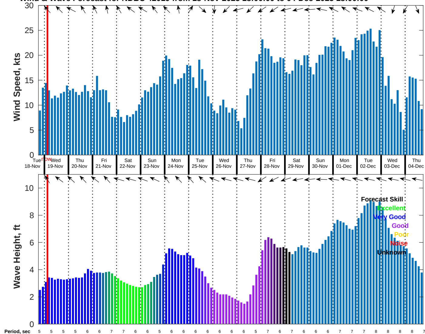
Wind & Wave Forecast for NDBC 42019 from 18-Nov-2025 18:00:00 to 04-Dec-2025 18:00:00
