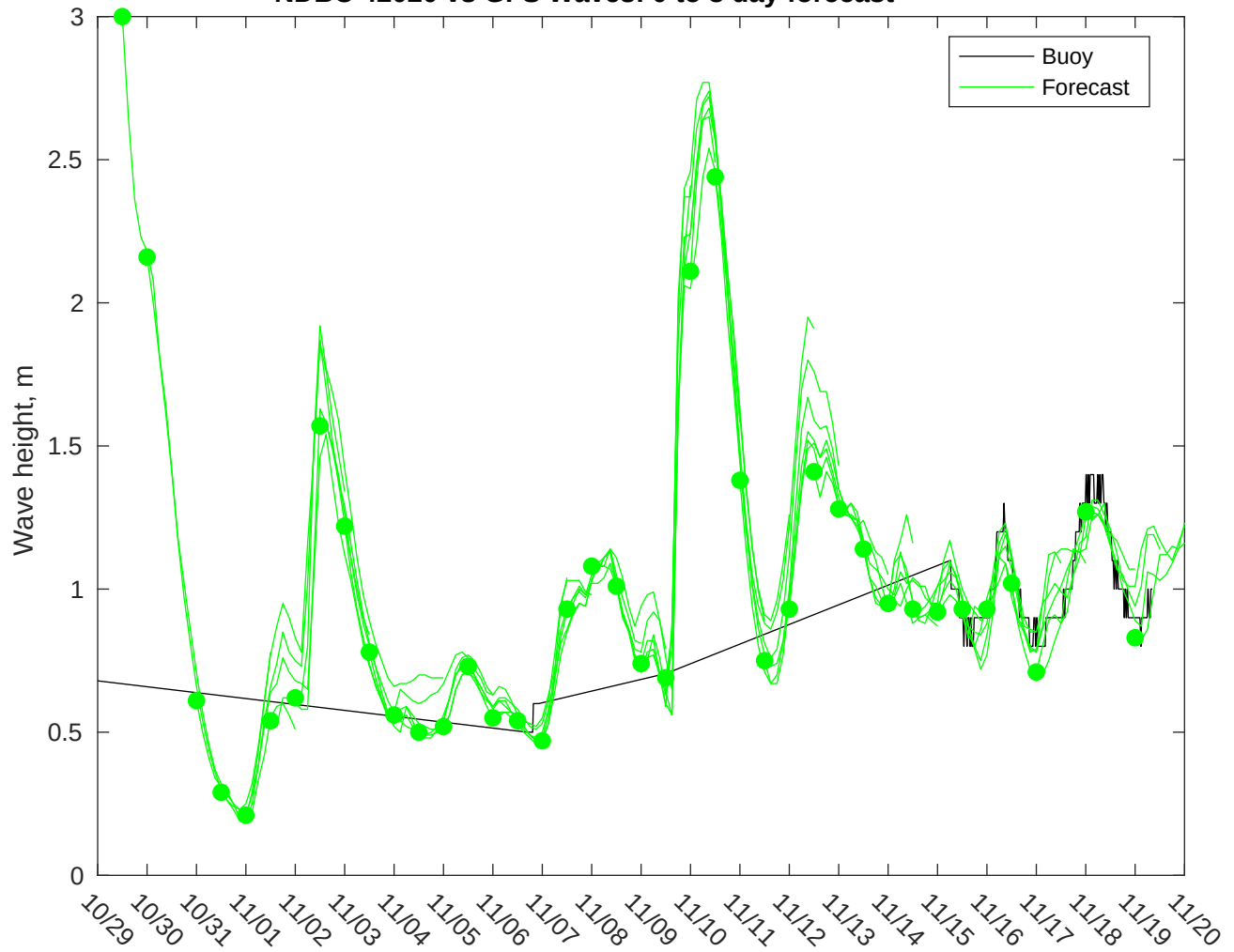
NDBC 42020 vs GFS Waves: 0 to 3 day forecast
