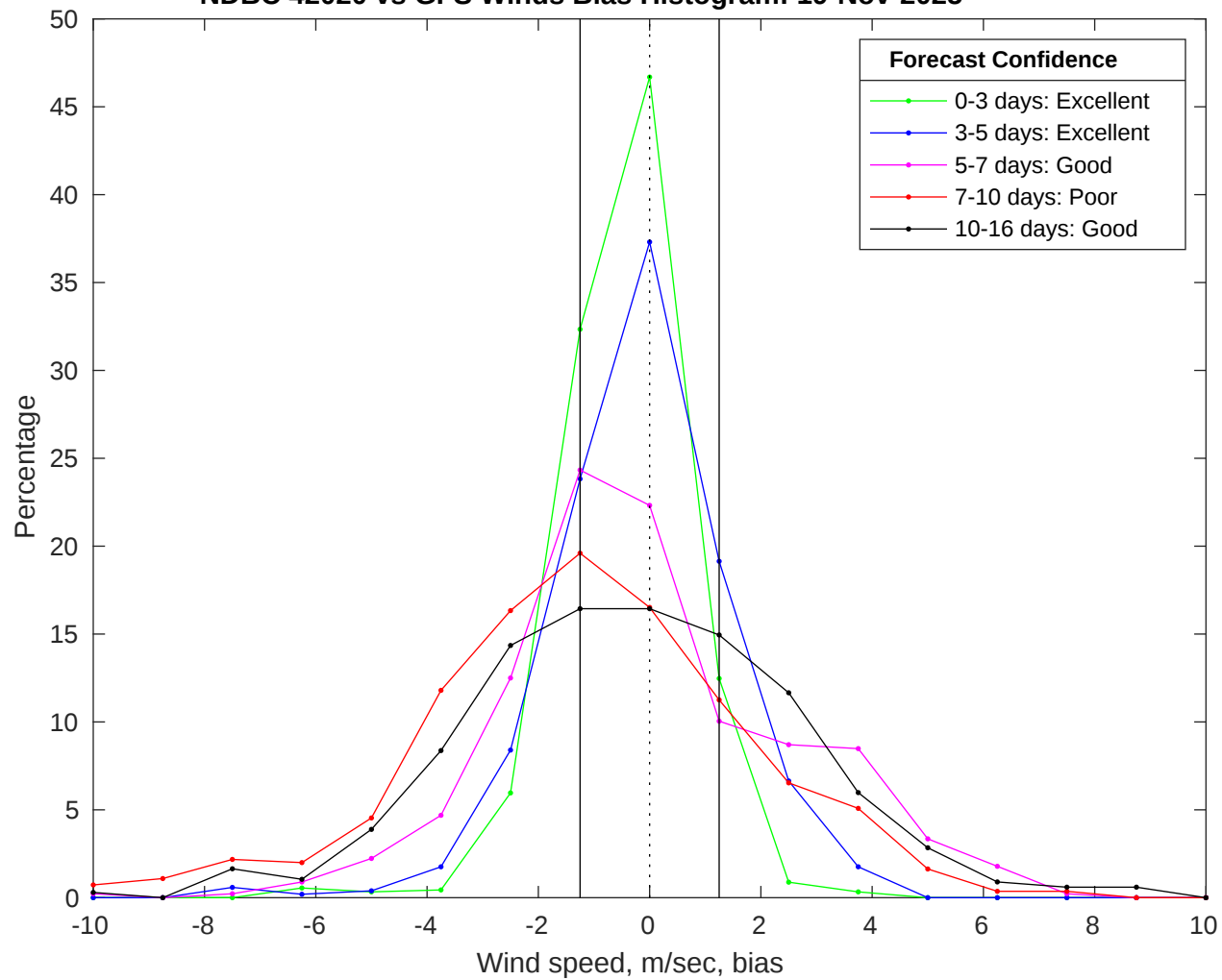
NDBC 42020 vs GFS Winds Bias Histogram: 19-Nov-2025
