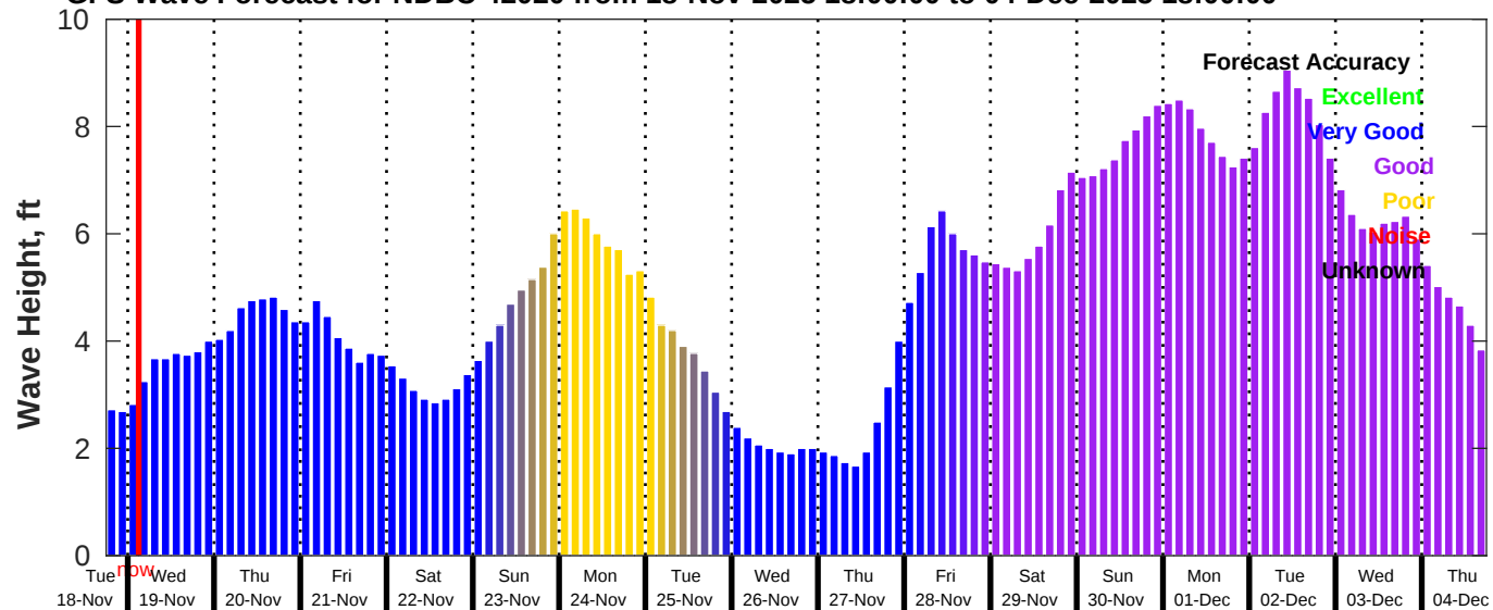
GFS Wave Forecast for NDBC 42020 from 18-Nov-2025 18:00:00 to 04-Dec-2025 18:00:00
