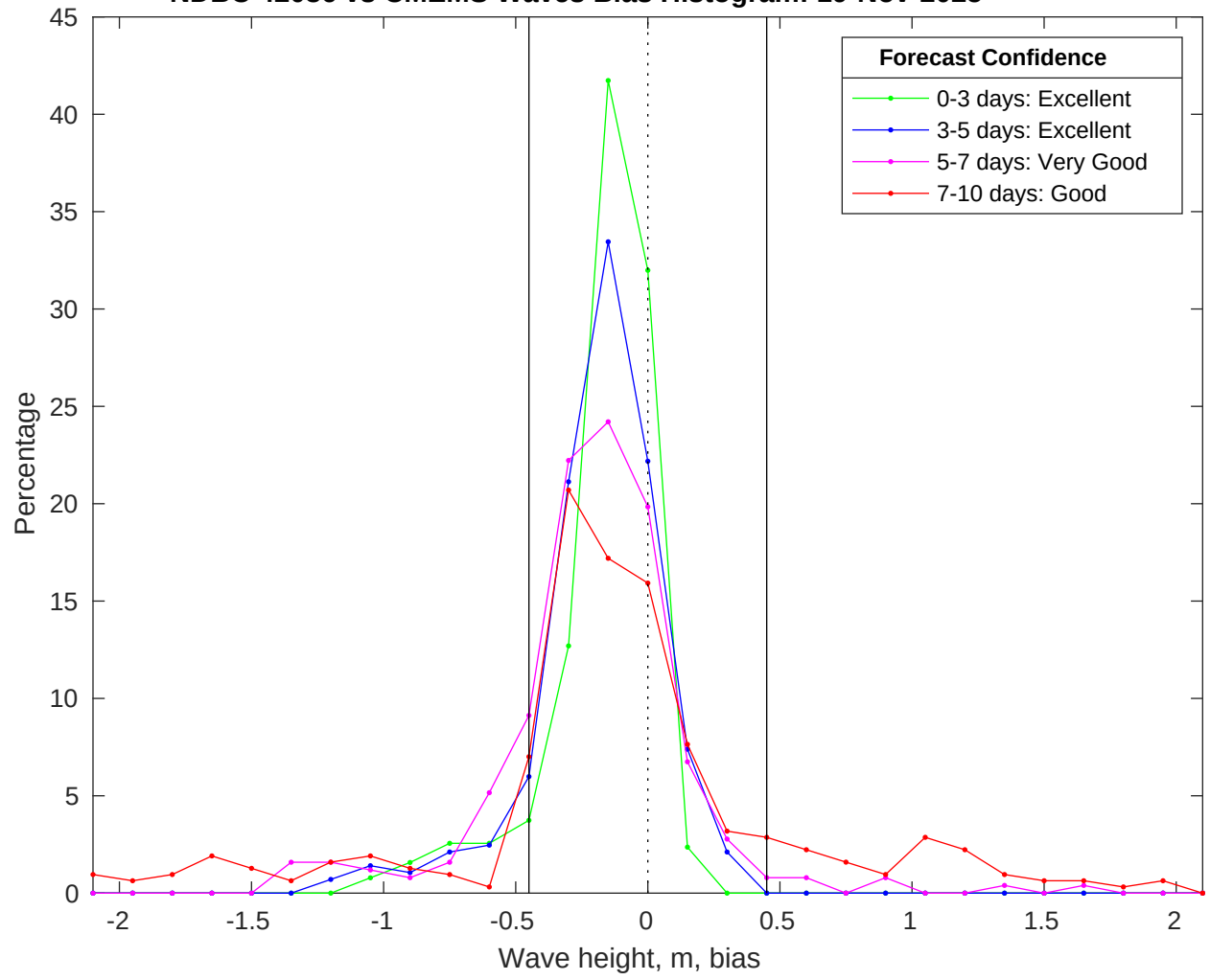
NDBC 42036 vs CMEMS Waves Bias Histogram: 19-Nov-2025
