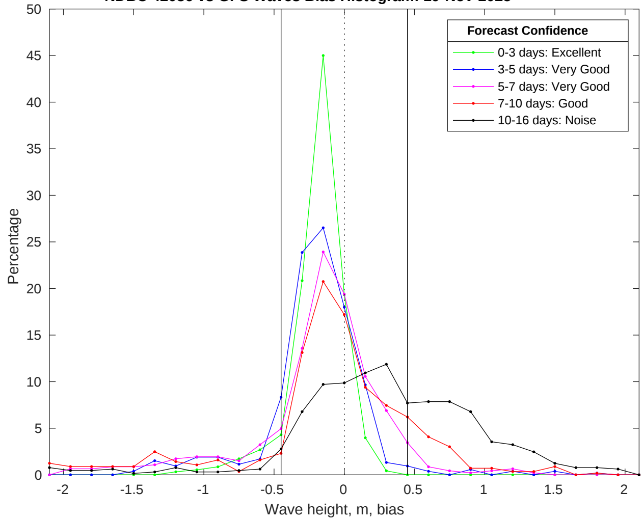
NDBC 42036 vs GFS Waves Bias Histogram: 19-Nov-2025
