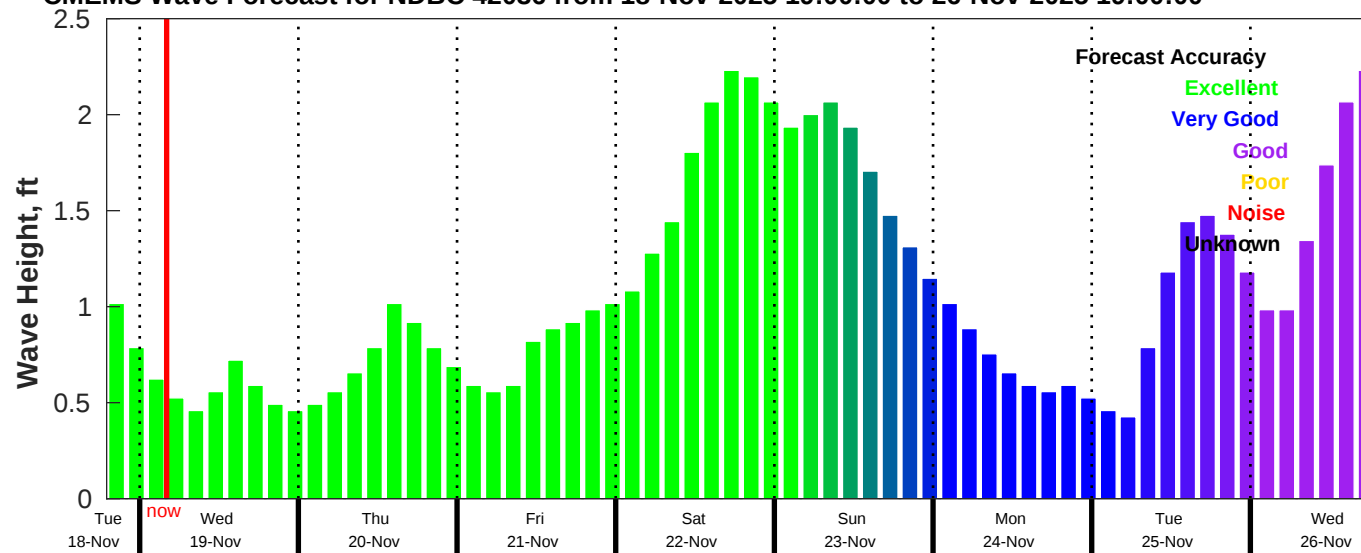
CMEMS Wave Forecast for NDBC 42036 from 18-Nov-2025 19:00:00 to 26-Nov-2025 19:00:00
