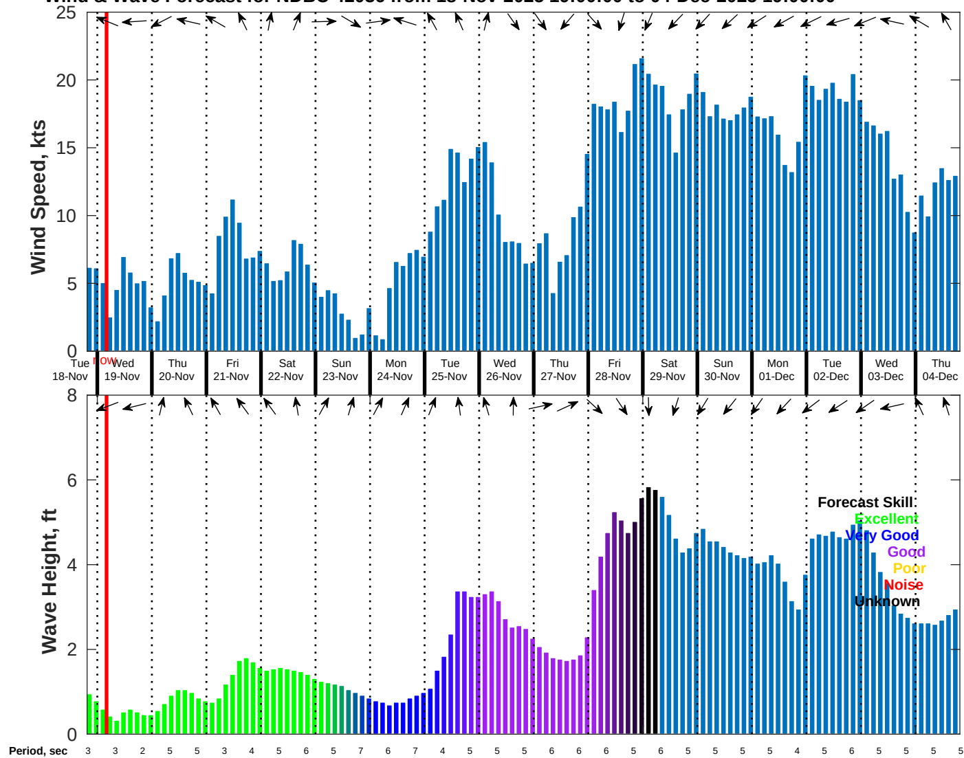
Wind & Wave Forecast for NDBC 42036 from 18-Nov-2025 19:00:00 to 04-Dec-2025 19:00:00
