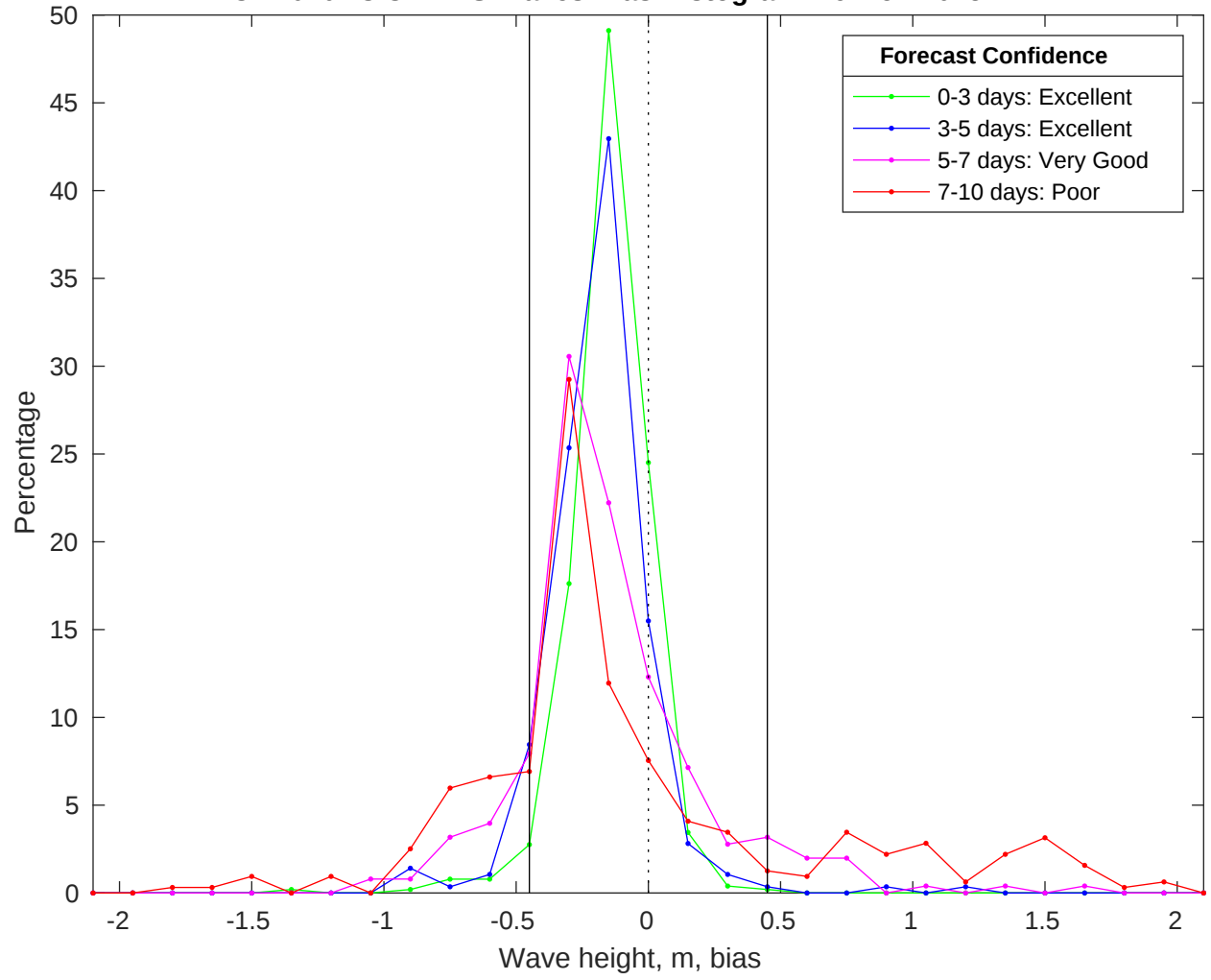
NDBC 42040 vs CMEMS Waves Bias Histogram: 19-Nov-2025
