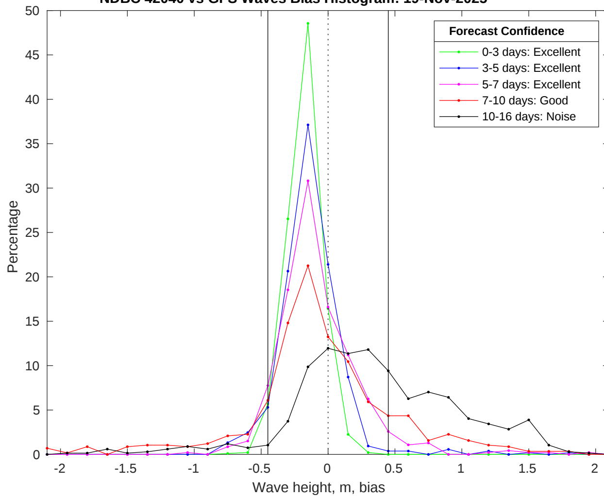
NDBC 42040 vs GFS Waves Bias Histogram: 19-Nov-2025
