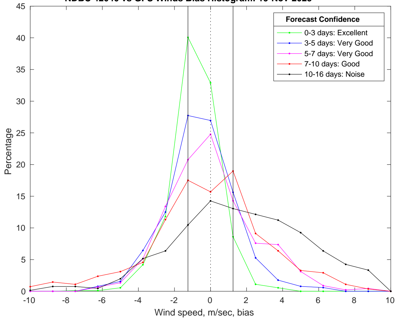
NDBC 42040 vs GFS Winds Bias Histogram: 19-Nov-2025
