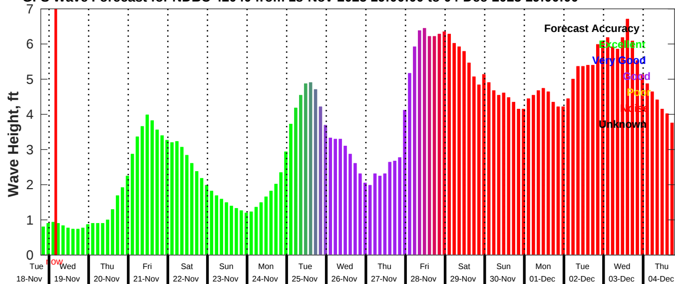
GFS Wave Forecast for NDBC 42040 from 18-Nov-2025 19:00:00 to 04-Dec-2025 19:00:00
