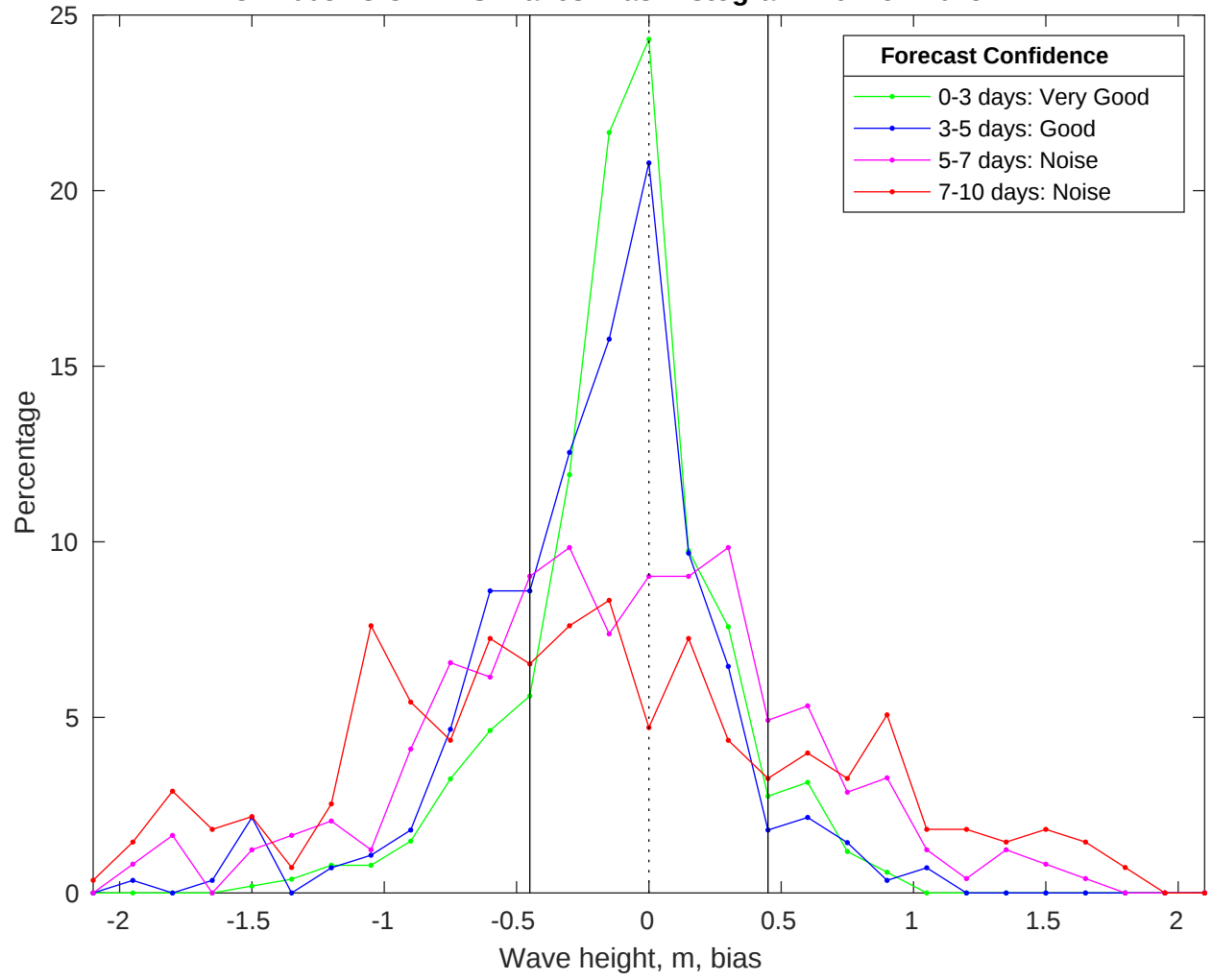
NDBC 44008 vs CMEMS Waves Bias Histogram: 19-Nov-2025
