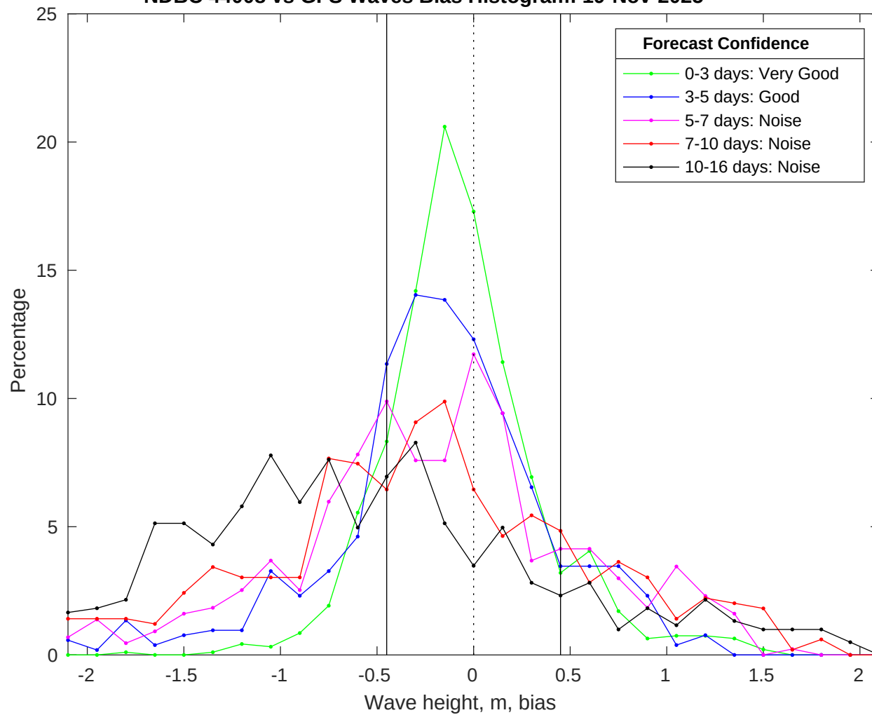
NDBC 44008 vs GFS Waves Bias Histogram: 19-Nov-2025
