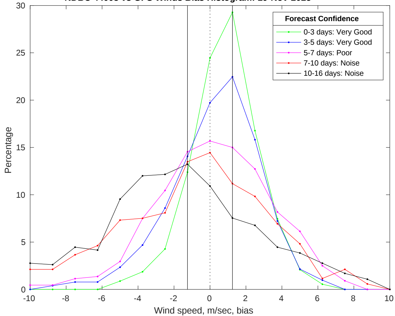
NDBC 44008 vs GFS Winds Bias Histogram: 19-Nov-2025
