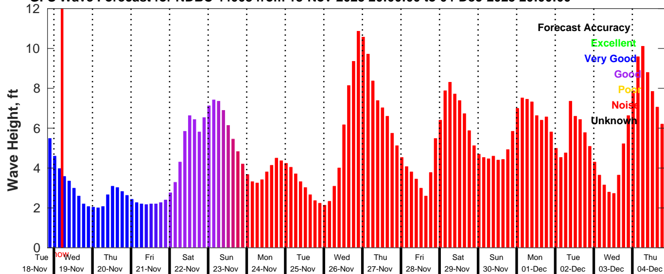
GFS Wave Forecast for NDBC 44008 from 18-Nov-2025 20:00:00 to 04-Dec-2025 20:00:00
