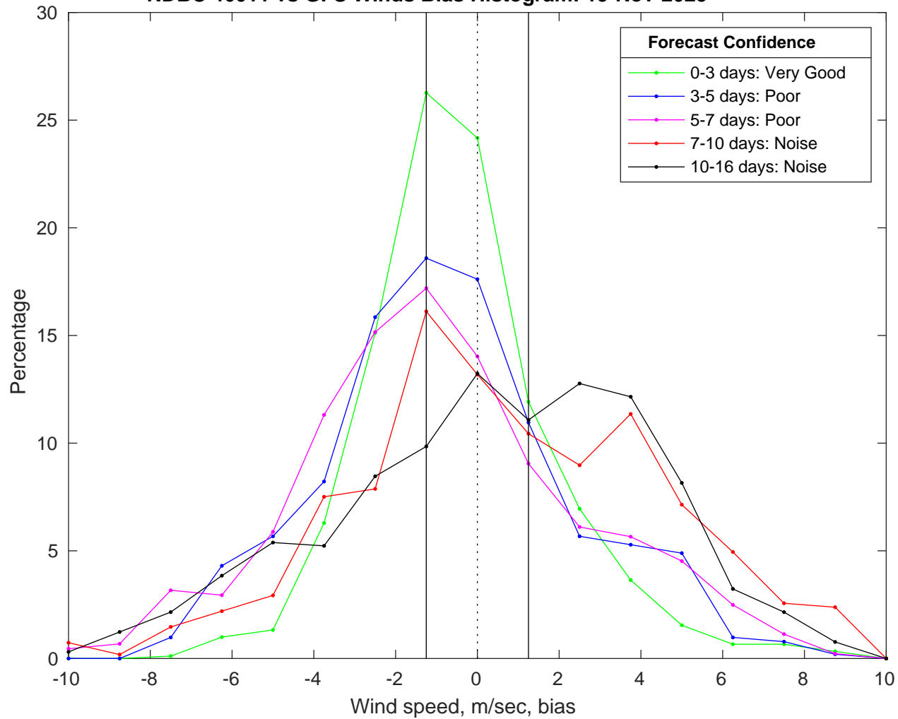
NDBC 46011 vs GFS Winds Bias Histogram: 19-Nov-2025
