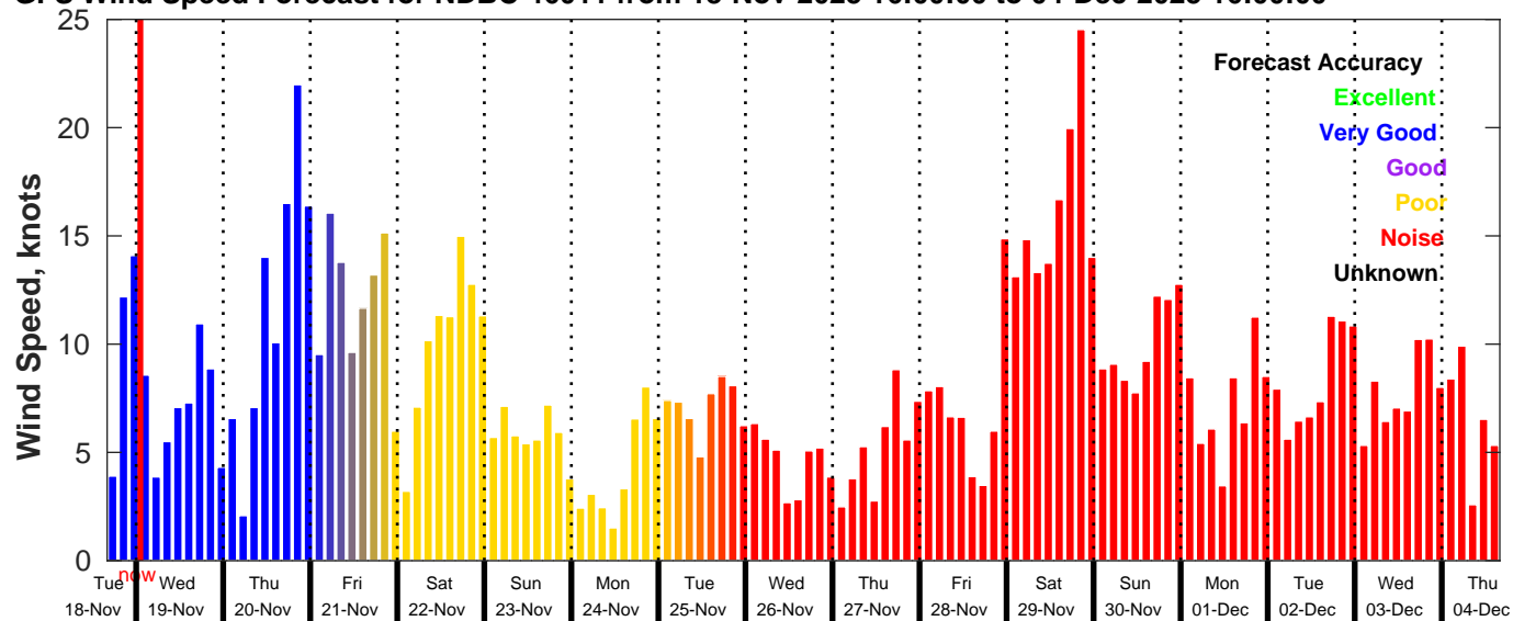
GFS Wind Speed Forecast for NDBC 46011 from 18-Nov-2025 16:00:00 to 04-Dec-2025 16:00:00
