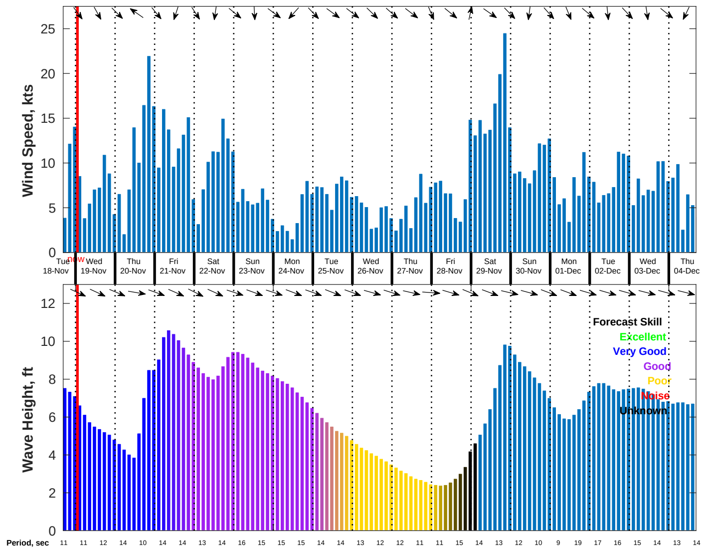
Wind & Wave Forecast for NDBC 46011 from 18-Nov-2025 16:00:00 to 04-Dec-2025 16:00:00
