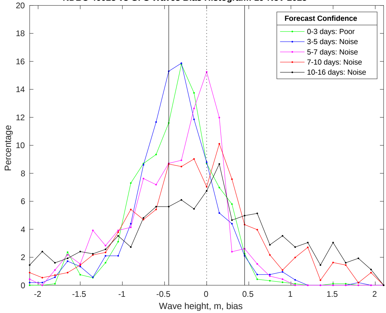
NDBC 46028 vs GFS Waves Bias Histogram: 19-Nov-2025
