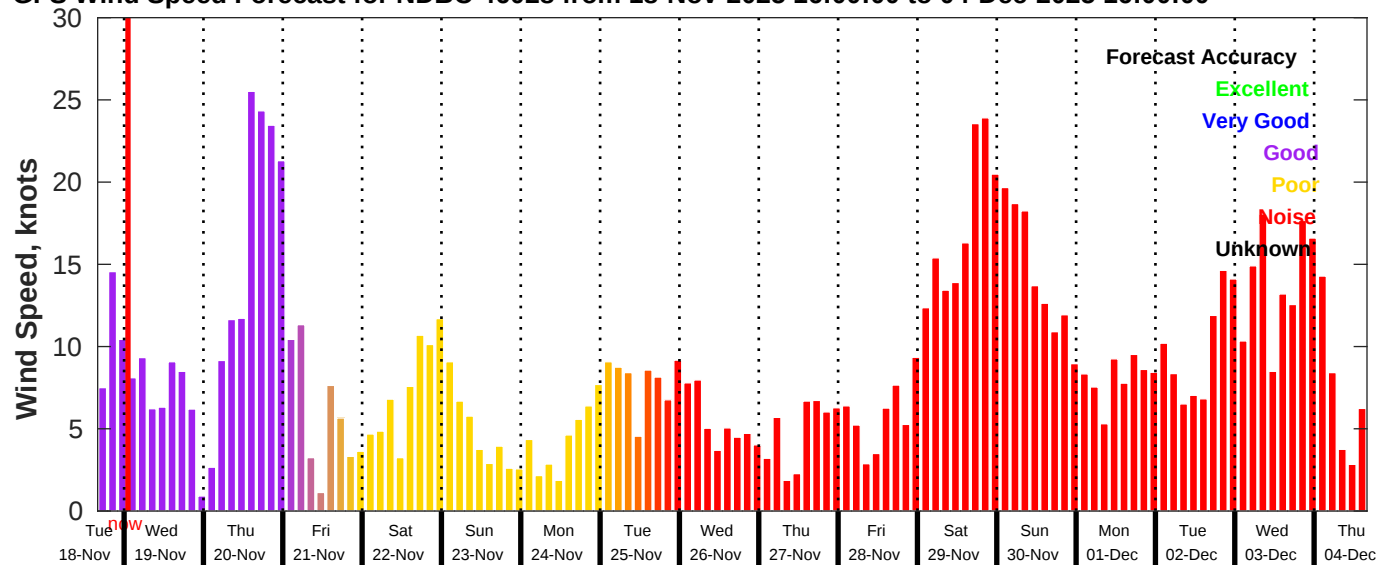
GFS Wind Speed Forecast for NDBC 46028 from 18-Nov-2025 16:00:00 to 04-Dec-2025 16:00:00
