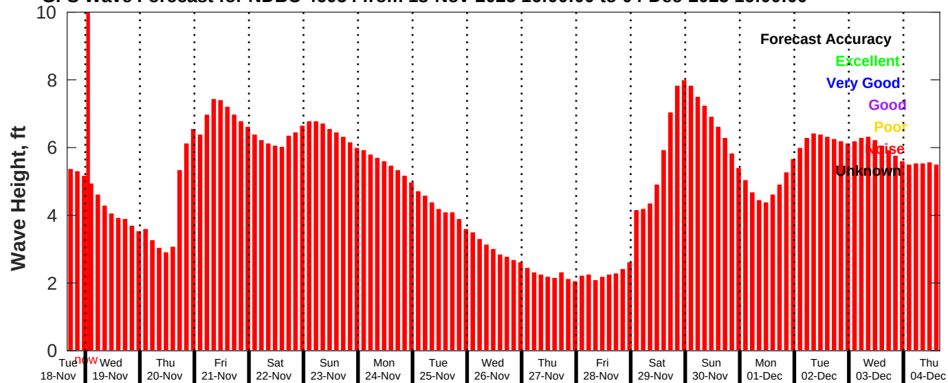
GFS Wave Forecast for NDBC 46054 from 18-Nov-2025 16:00:00 to 04-Dec-2025 16:00:00
