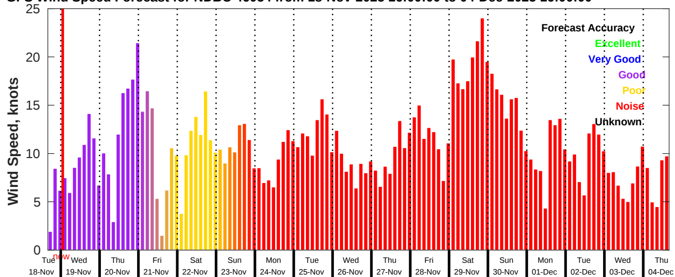
GFS Wind Speed Forecast for NDBC 46054 from 18-Nov-2025 16:00:00 to 04-Dec-2025 16:00:00
