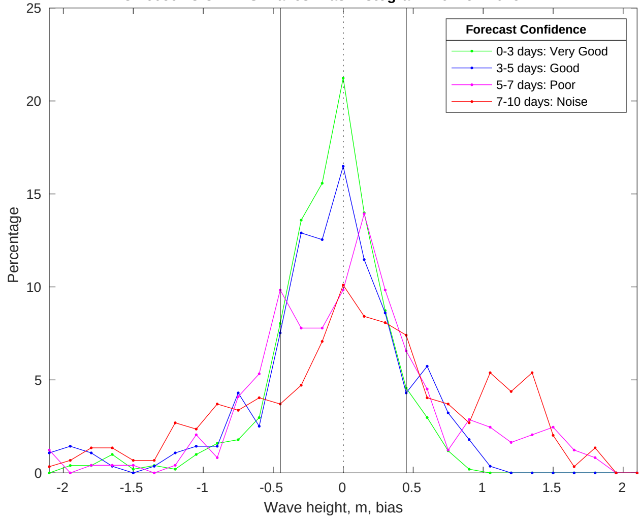
NDBC 46059 vs CMEMS Waves Bias Histogram: 19-Nov-2025
