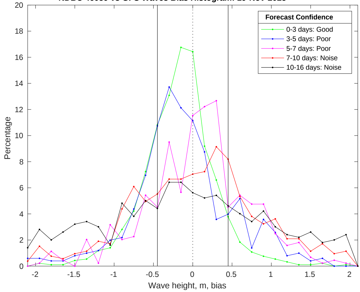
NDBC 46059 vs GFS Waves Bias Histogram: 19-Nov-2025
