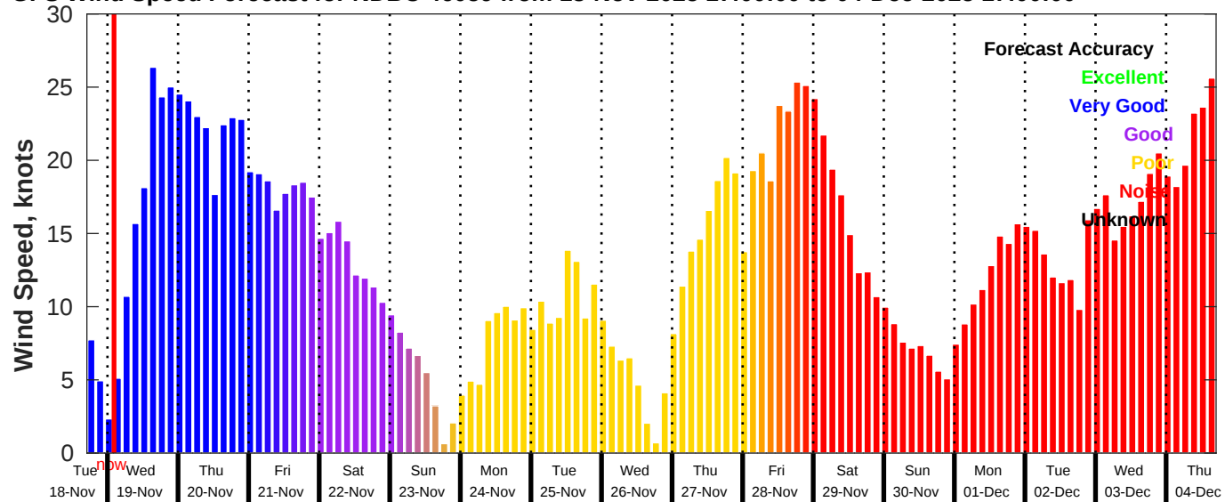
GFS Wind Speed Forecast for NDBC 46059 from 18-Nov-2025 17:00:00 to 04-Dec-2025 17:00:00
