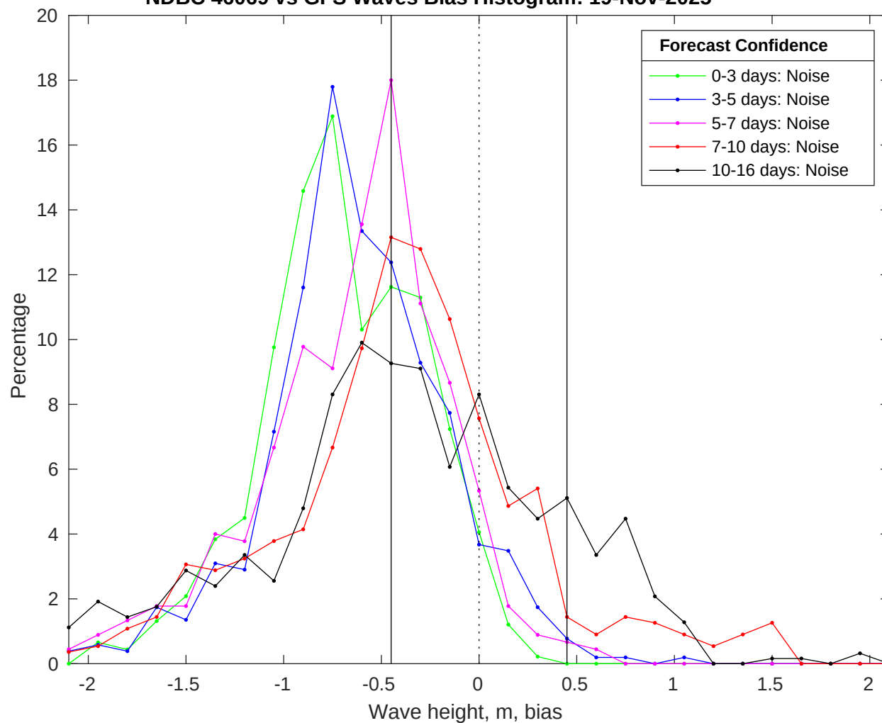
NDBC 46069 vs GFS Waves Bias Histogram: 19-Nov-2025
