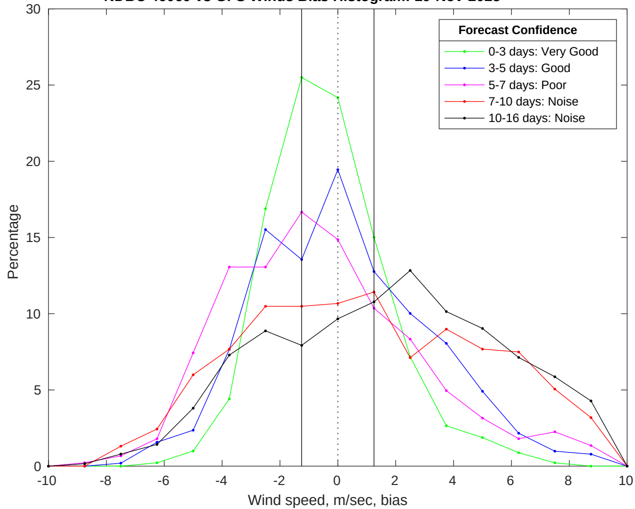
NDBC 46069 vs GFS Winds Bias Histogram: 19-Nov-2025
