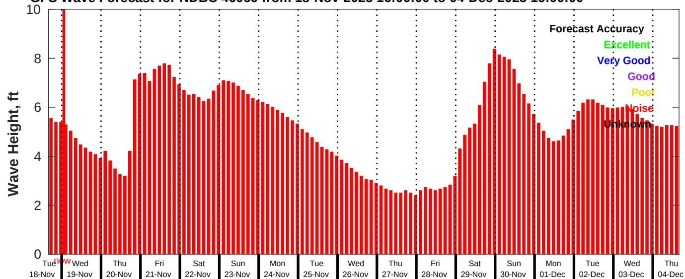
GFS Wave Forecast for NDBC 46069 from 18-Nov-2025 16:00:00 to 04-Dec-2025 16:00:00
