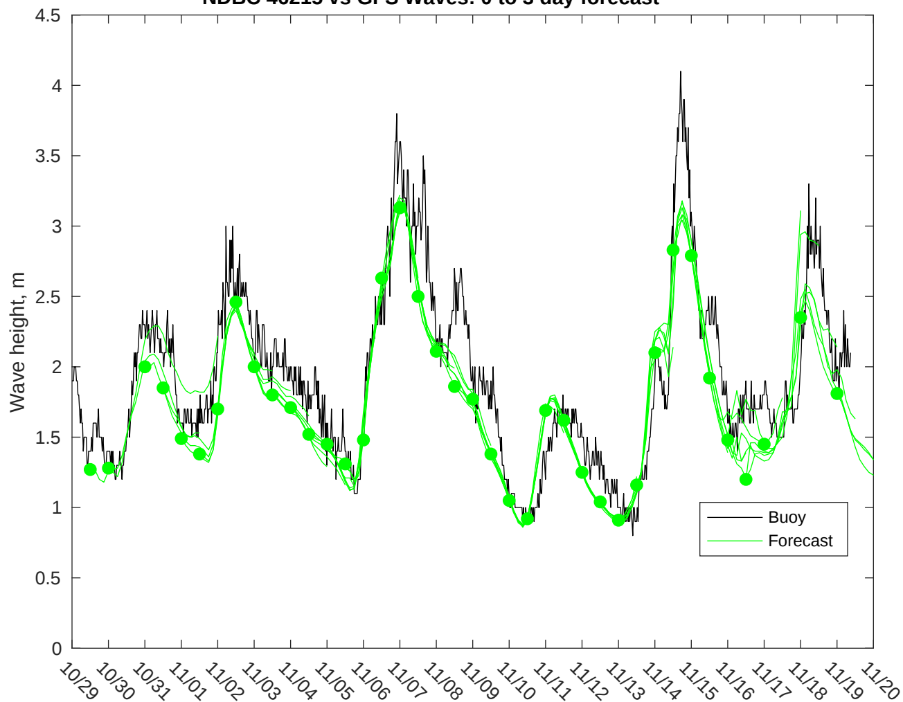
NDBC 46215 vs GFS Waves: 0 to 3 day forecast
