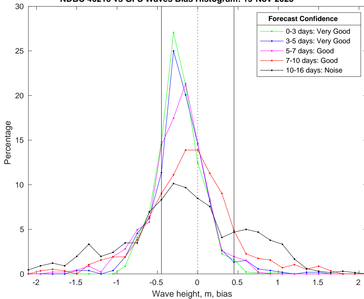
NDBC 46215 vs GFS Waves Bias Histogram: 19-Nov-2025
