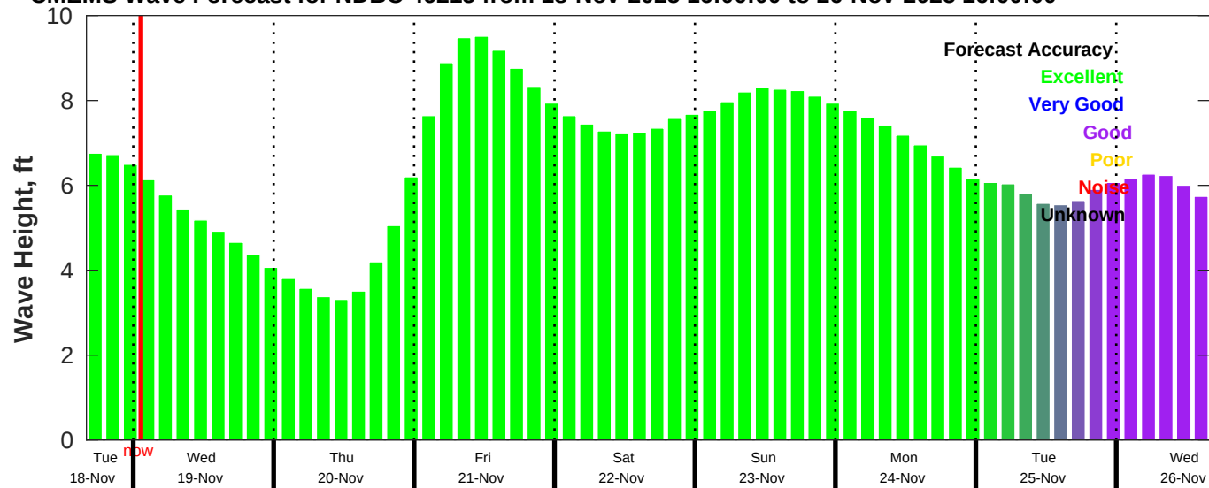
CMEMS Wave Forecast for NDBC 46215 from 18-Nov-2025 16:00:00 to 26-Nov-2025 16:00:00
