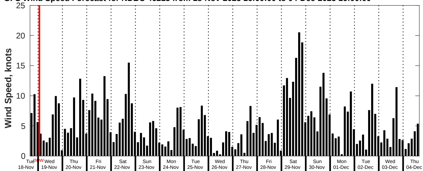
GFS Wind Speed Forecast for NDBC 46215 from 18-Nov-2025 16:00:00 to 04-Dec-2025 16:00:00
