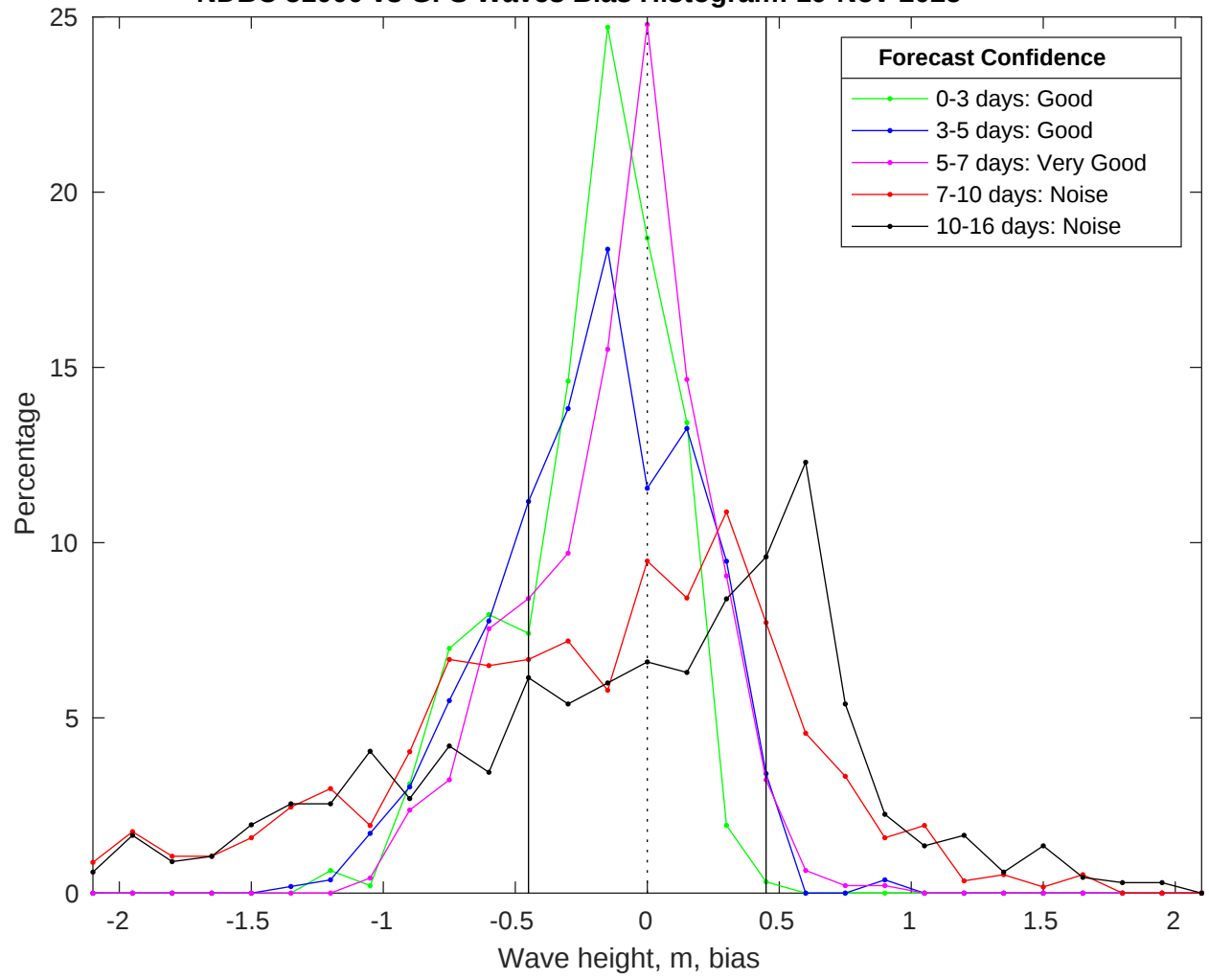
NDBC 51000 vs GFS Waves Bias Histogram: 19-Nov-2025
