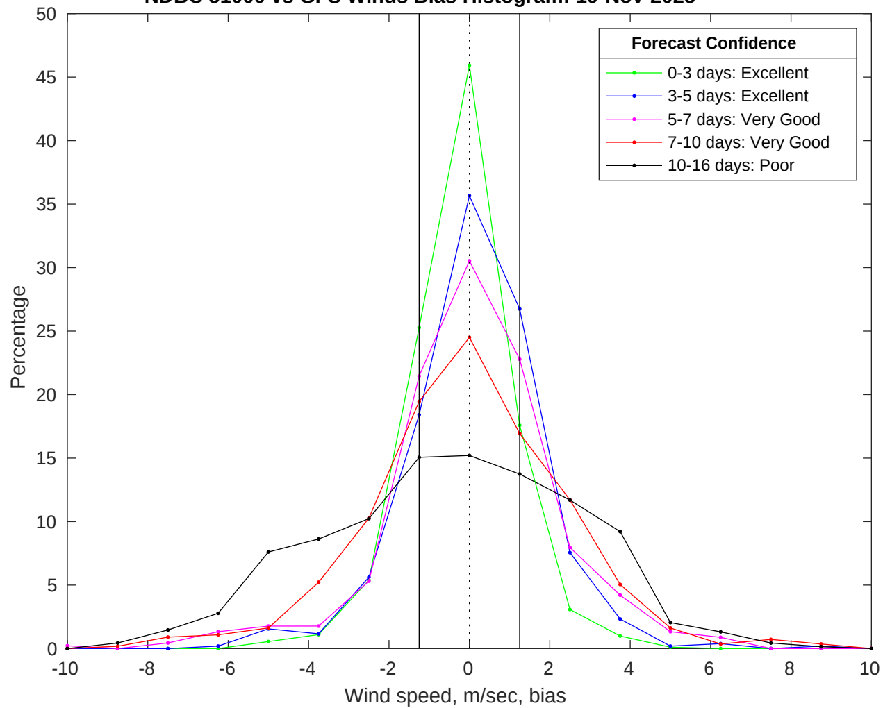
NDBC 51000 vs GFS Winds Bias Histogram: 19-Nov-2025
