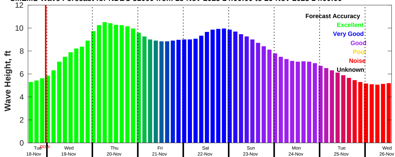
CMEMS Wave Forecast for NDBC 51000 from 18-Nov-2025 14:00:00 to 26-Nov-2025 14:00:00
