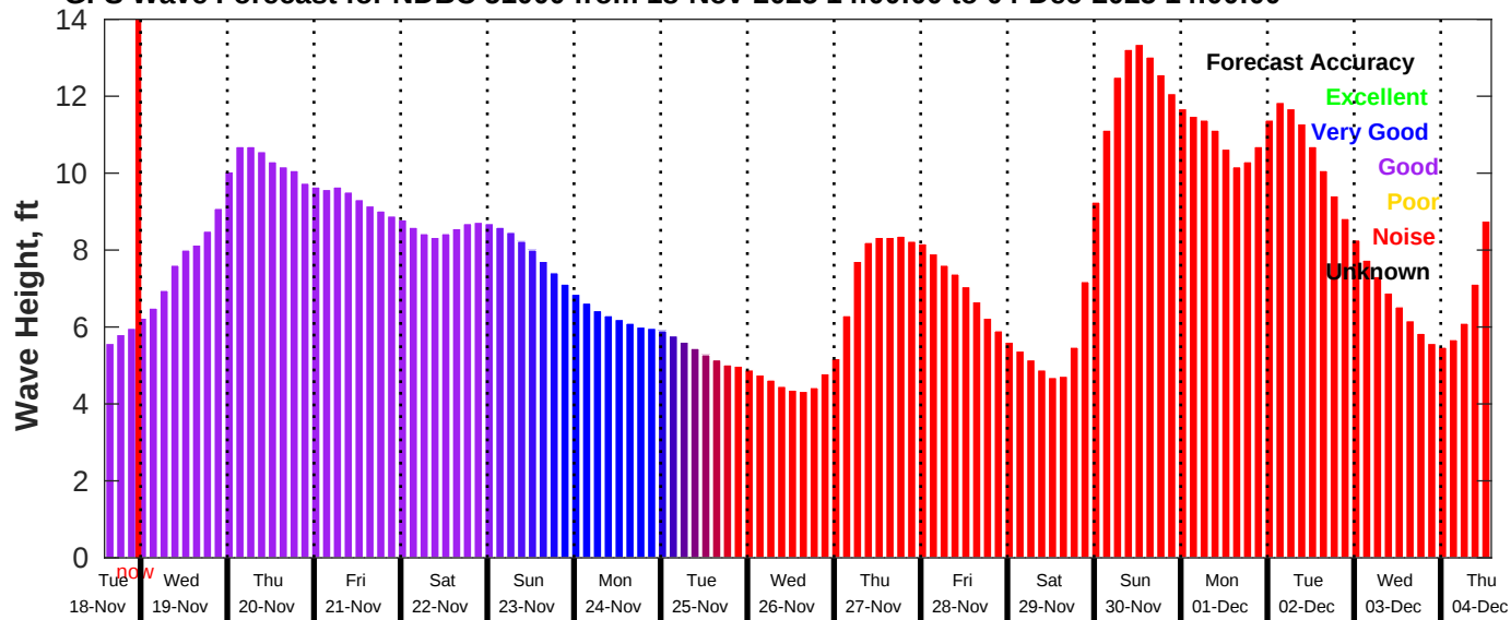
GFS Wave Forecast for NDBC 51000 from 18-Nov-2025 14:00:00 to 04-Dec-2025 14:00:00
