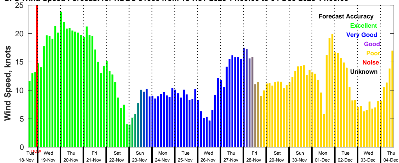
GFS Wind Speed Forecast for NDBC 51000 from 18-Nov-2025 14:00:00 to 04-Dec-2025 14:00:00
