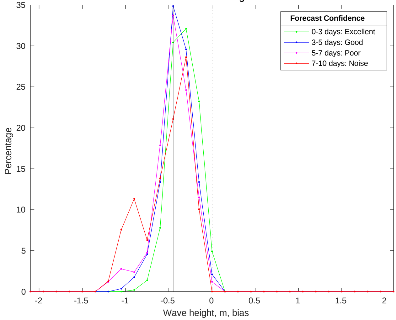
NDBC 51209 vs CMEMS Waves Bias Histogram: 19-Nov-2025
