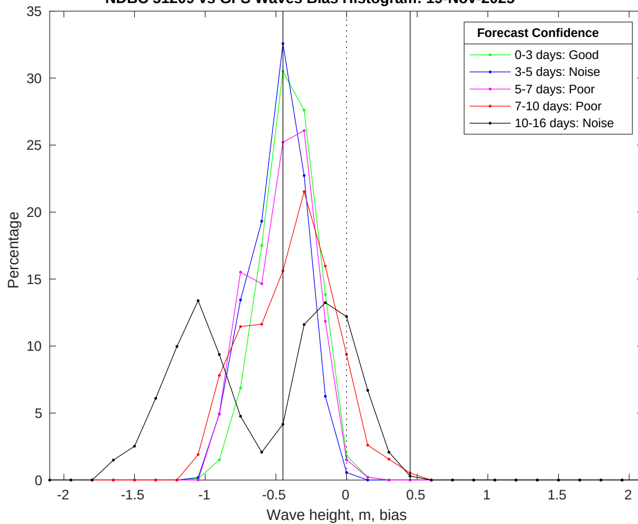
NDBC 51209 vs GFS Waves Bias Histogram: 19-Nov-2025
