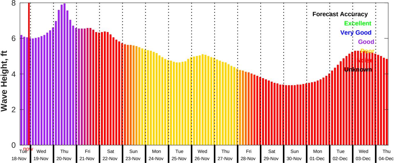
GFS Wave Forecast for NDBC 51209 from 18-Nov-2025 13:00:00 to 04-Dec-2025 13:00:00
