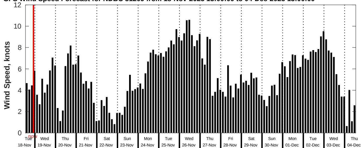
GFS Wind Speed Forecast for NDBC 51209 from 18-Nov-2025 13:00:00 to 04-Dec-2025 13:00:00
