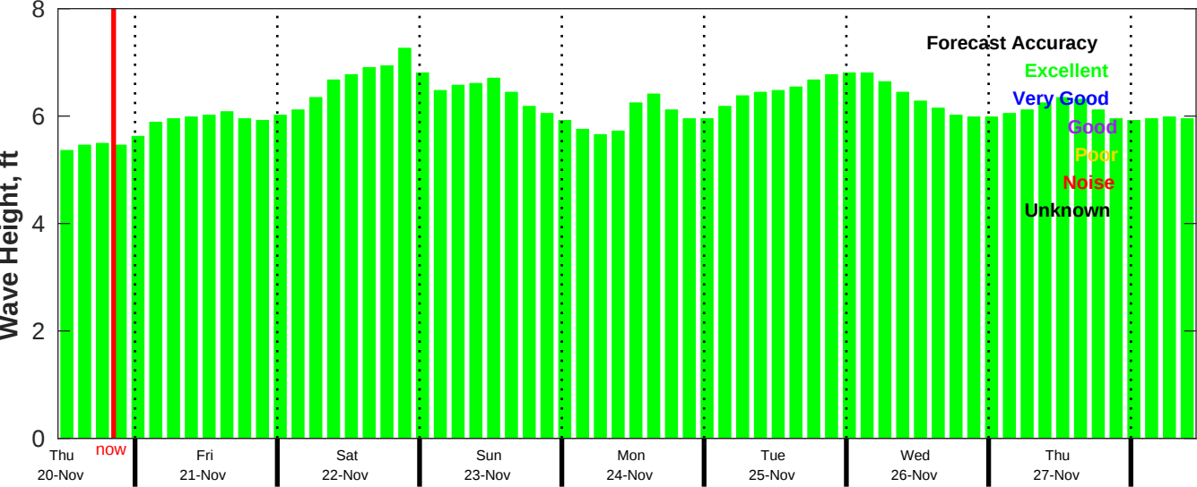
CMEMS Wave Forecast for NDBC 52211 from 19-Nov-2025 11:00:00 to 27-Nov-2025 11:00:00
