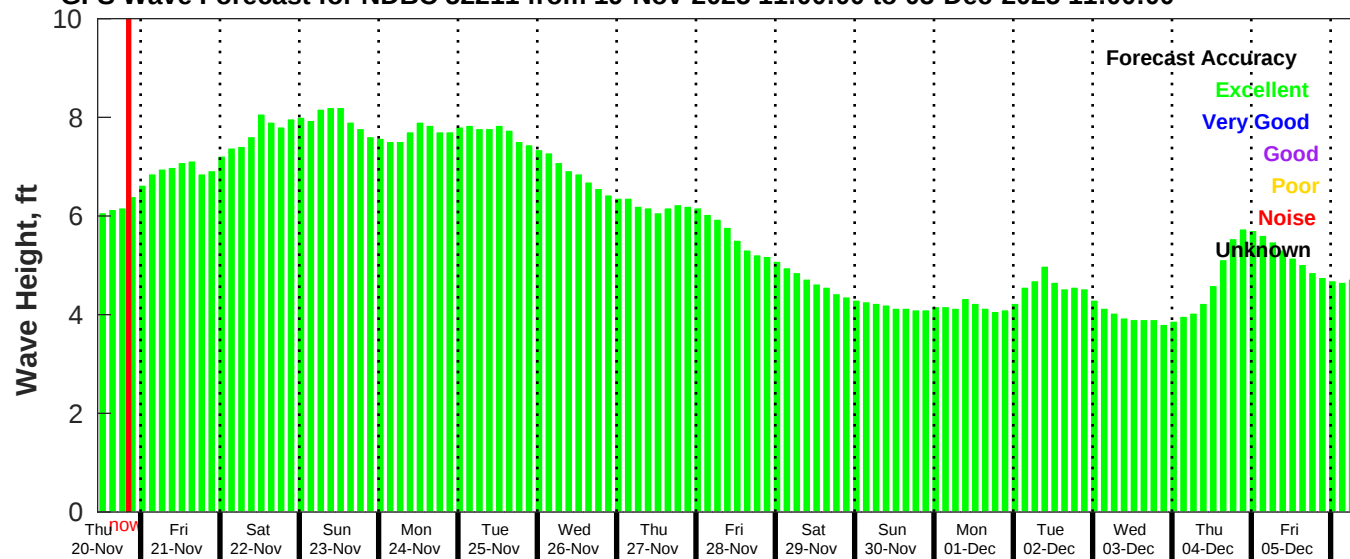
GFS Wave Forecast for NDBC 52211 from 19-Nov-2025 11:00:00 to 05-Dec-2025 11:00:00
