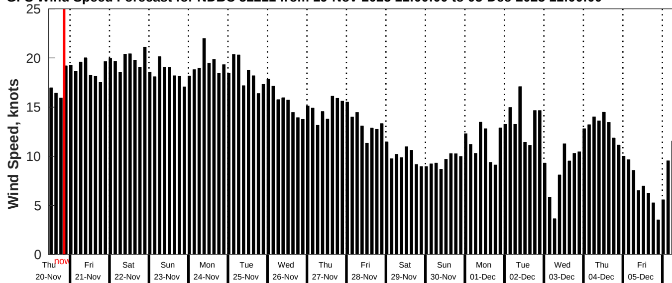
GFS Wind Speed Forecast for NDBC 52211 from 19-Nov-2025 11:00:00 to 05-Dec-2025 11:00:00
