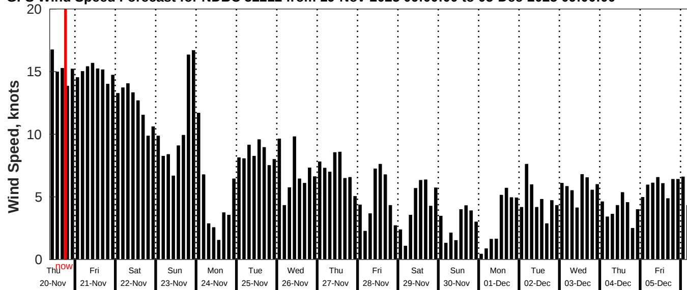
GFS Wind Speed Forecast for NDBC 52212 from 19-Nov-2025 09:00:00 to 05-Dec-2025 09:00:00
