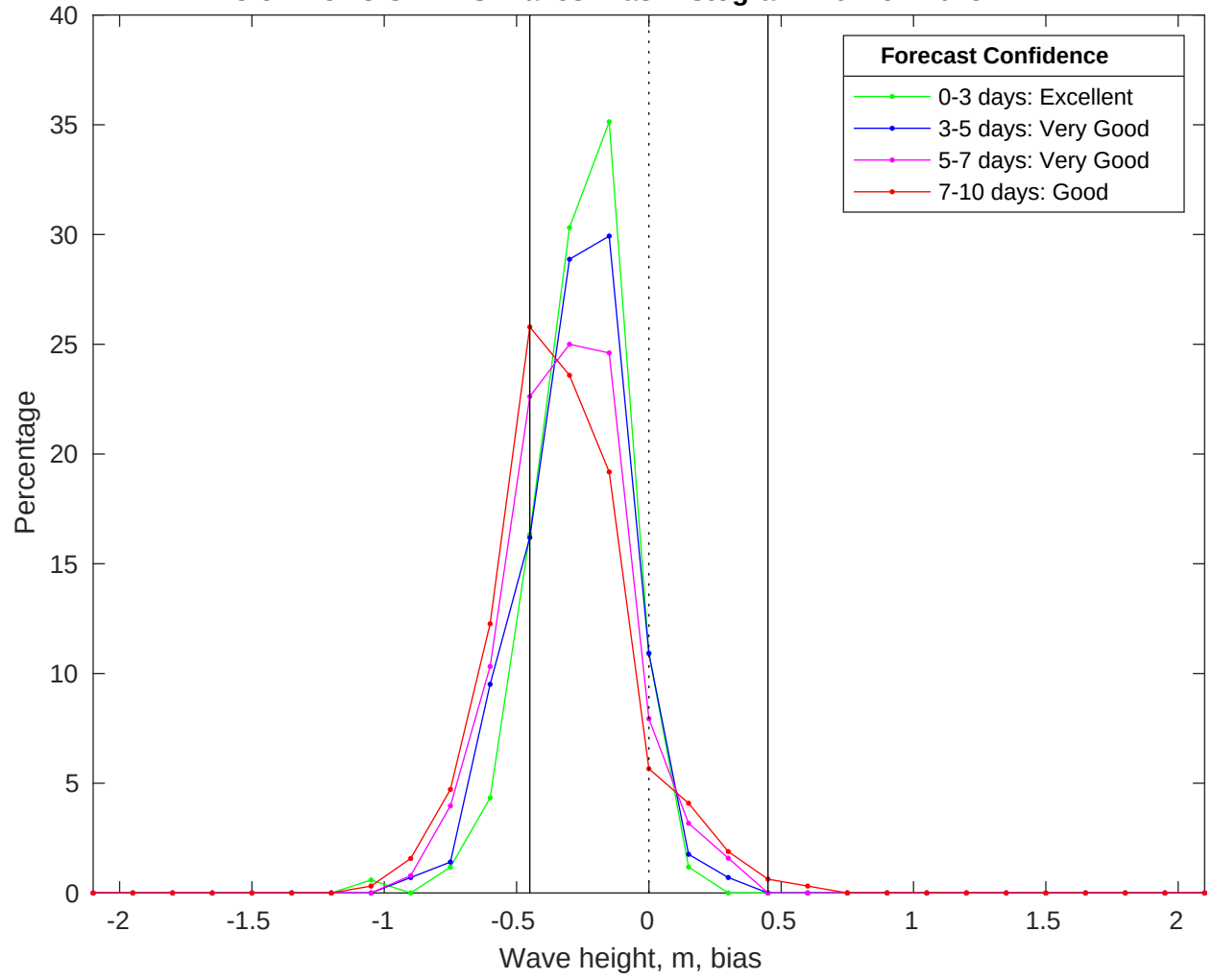
NDBC 52213 vs CMEMS Waves Bias Histogram: 19-Nov-2025
